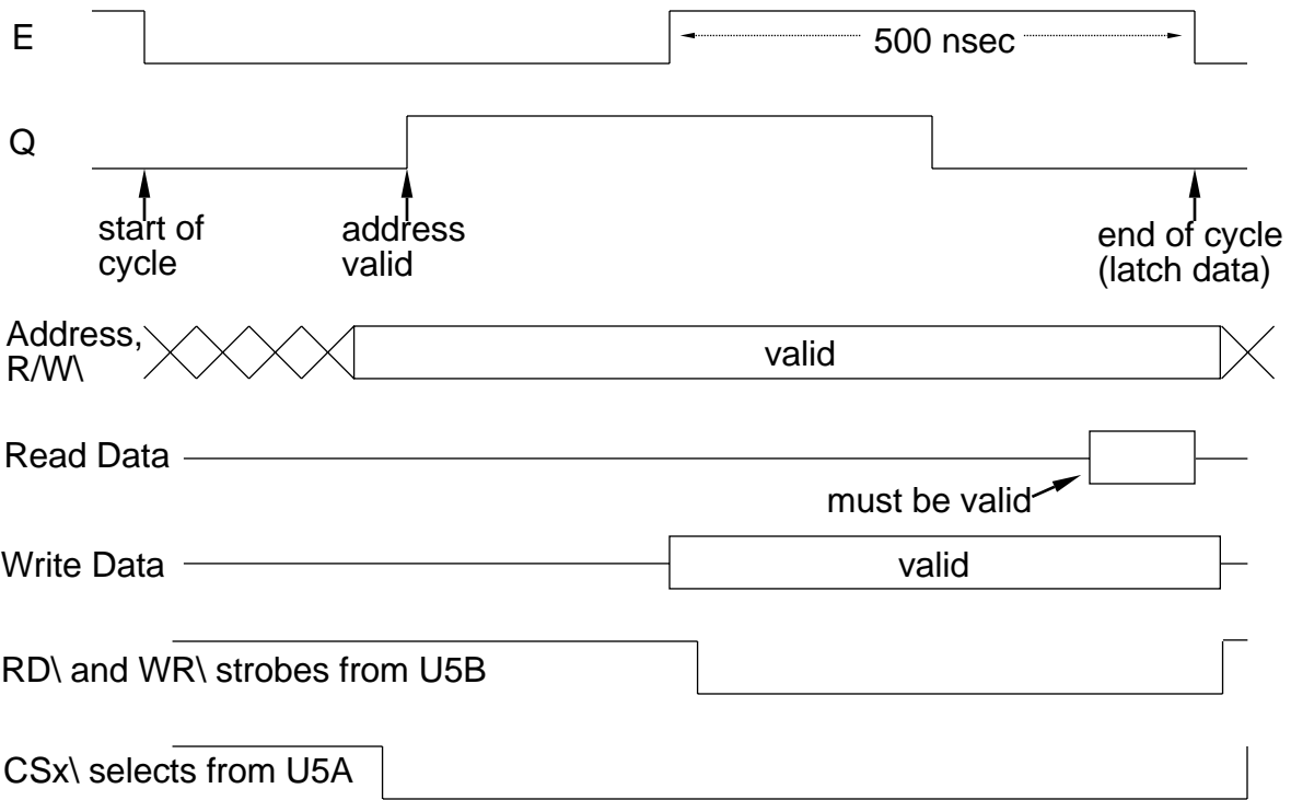
FIGURE 3. 6809 Memory Timing (4 MHz osc)
