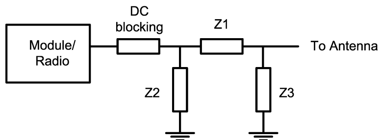
Figure 25. PI Network
