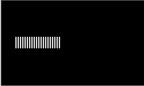
Figure C23: Effort Stimuli
