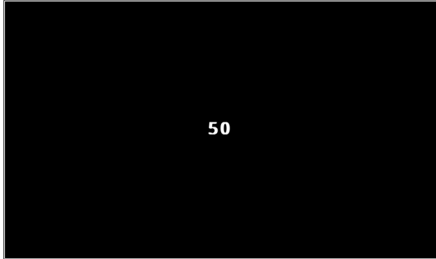
Figure C23: Effort Stimuli
