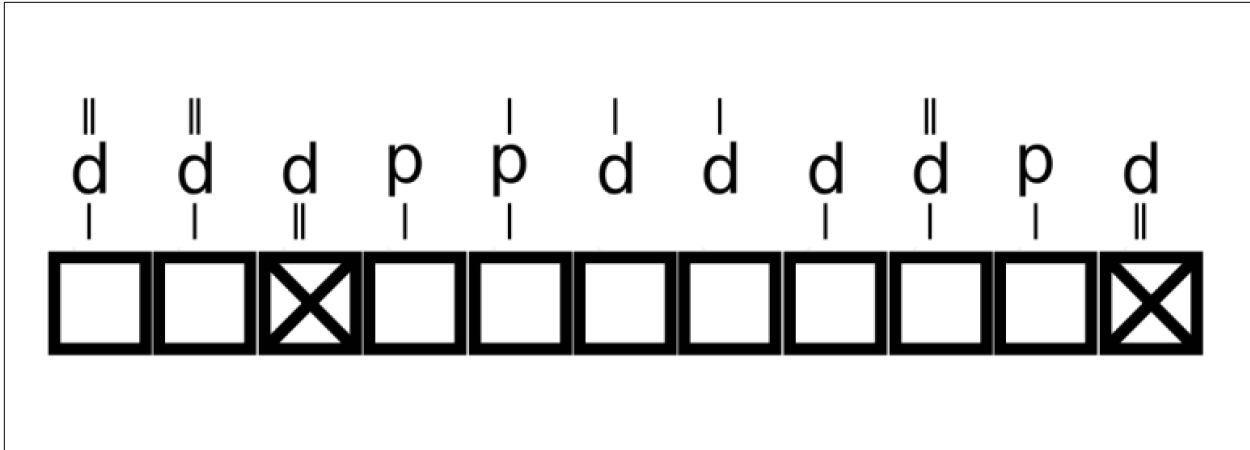
Figure C17: d2 Stimuli
