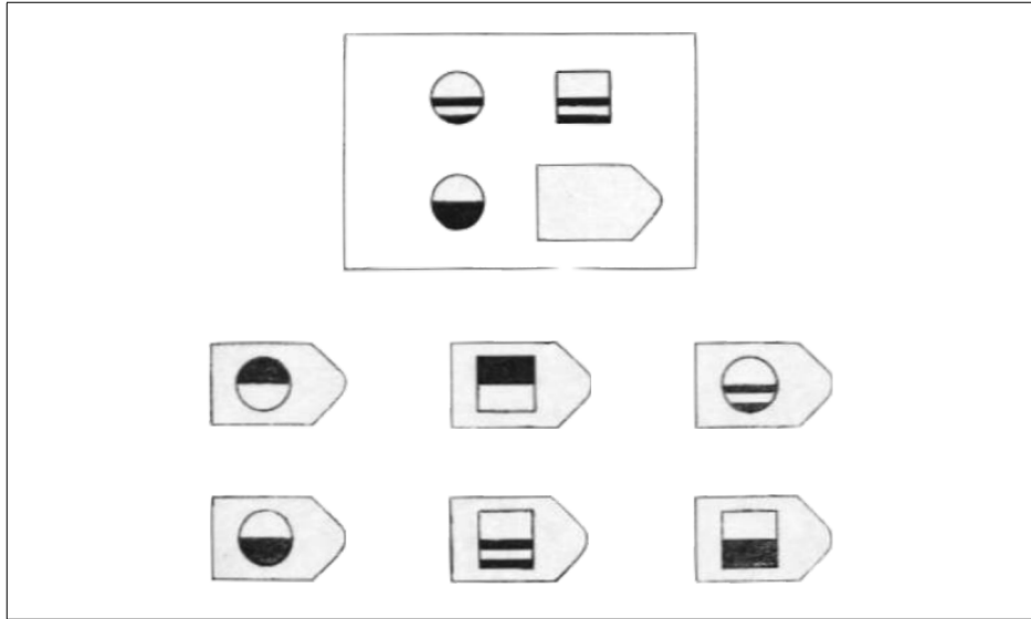
Figure C22: Raven's Stimulus
