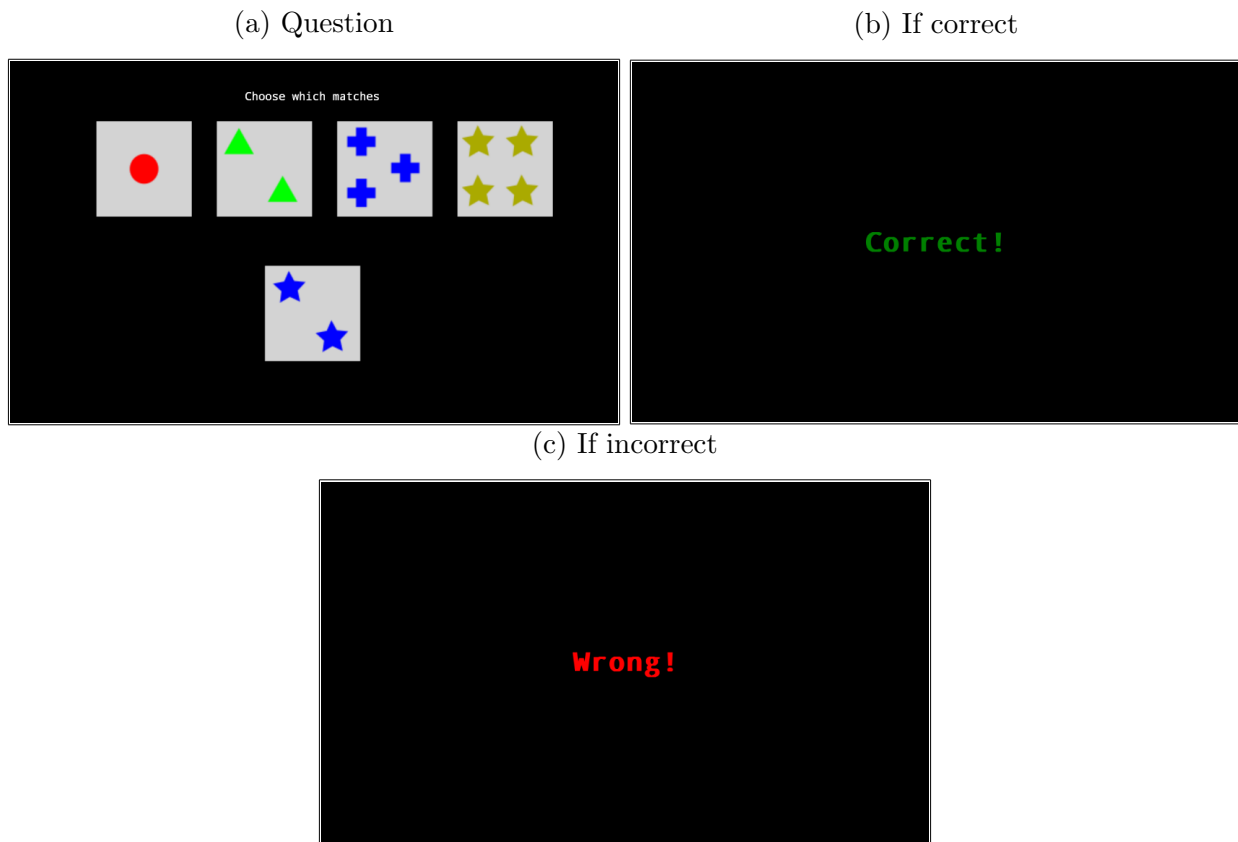
Figure C21: Wisconsin Stimuli
