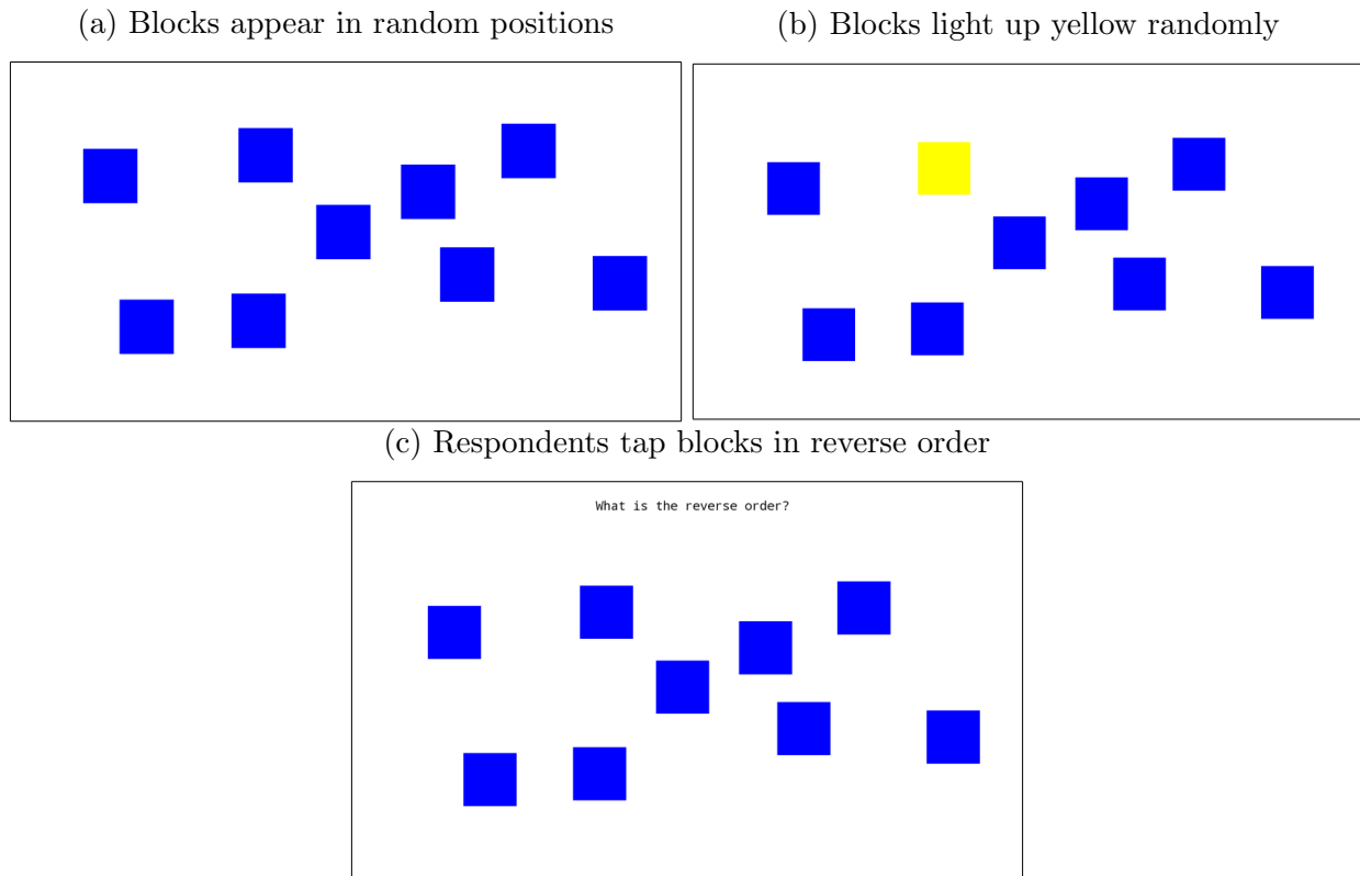
Figure C18: Corsi Stimuli
